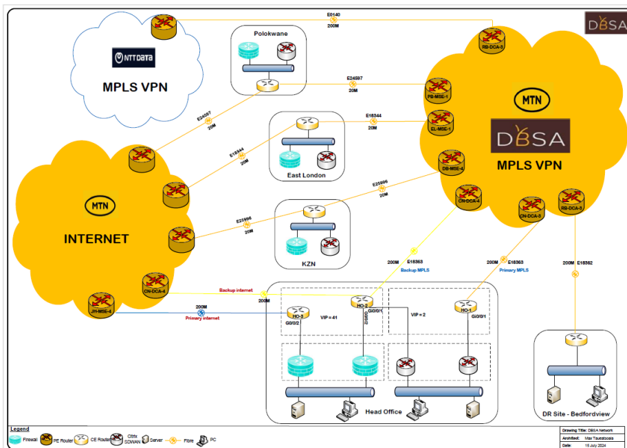
FIGURE 2: DBSA WAN ARCHITECTURE (MPLS AND DIA)
